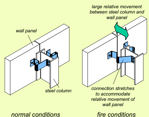
example of a flexible connection
