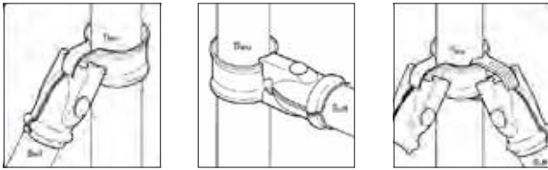
Rail Clamp
