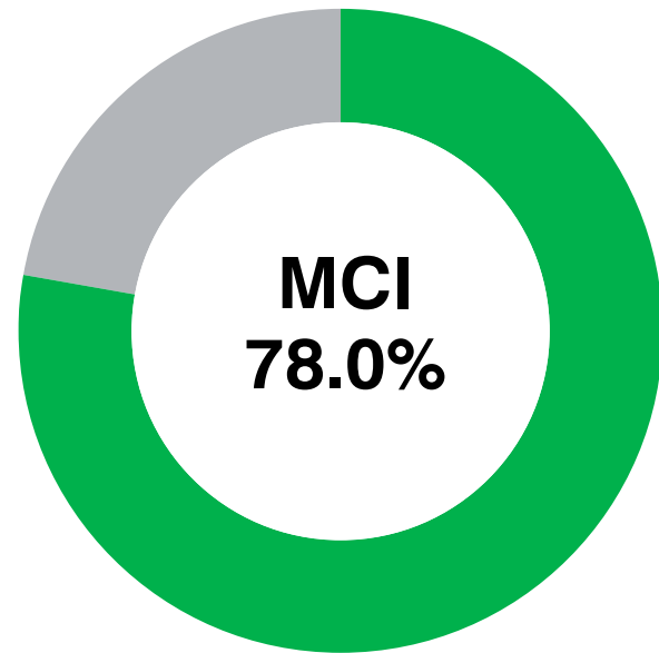
Figure 4. MCI score
